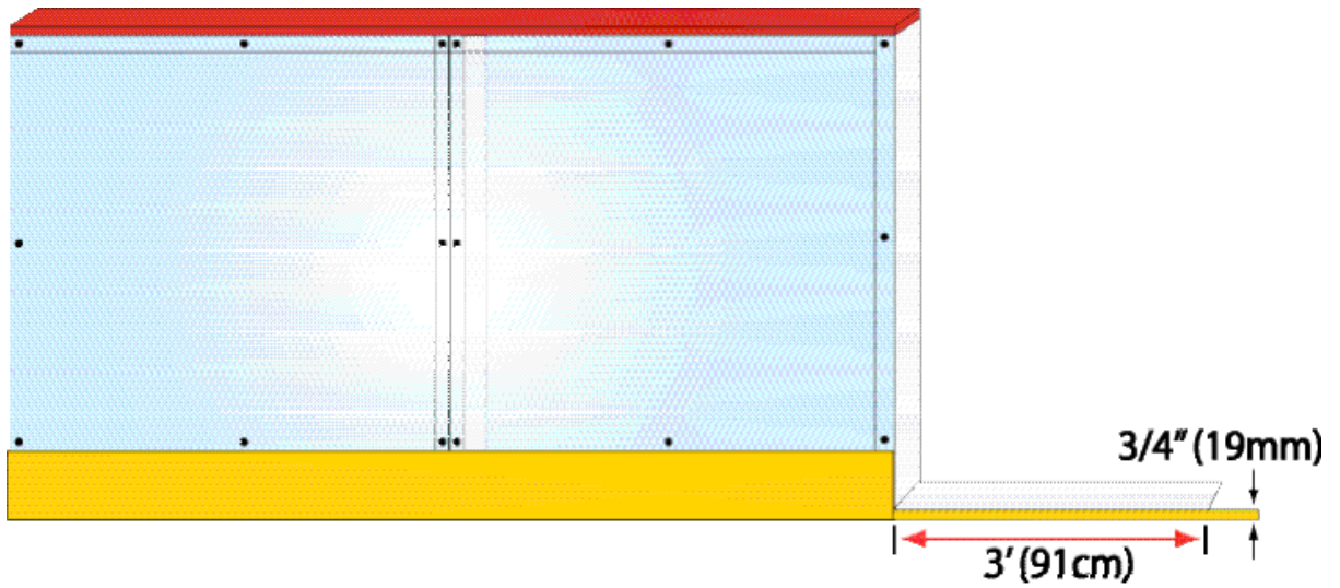
Figure 1: Boards with plexiglass, width of the doors and height of the kick plate at the doors.
